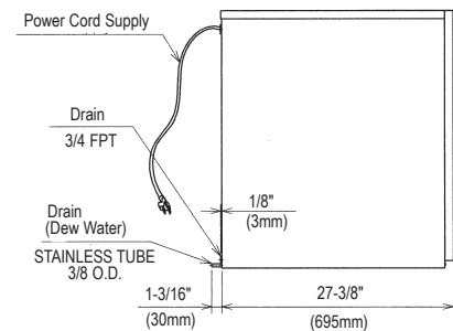
KM-500 SIDE VIEW
