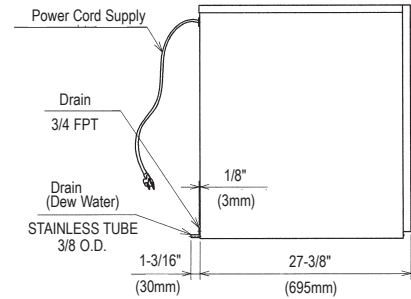
KM-280 SIDE VIEW
