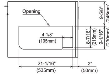
KM-280/500 ICE DROP ZONE
